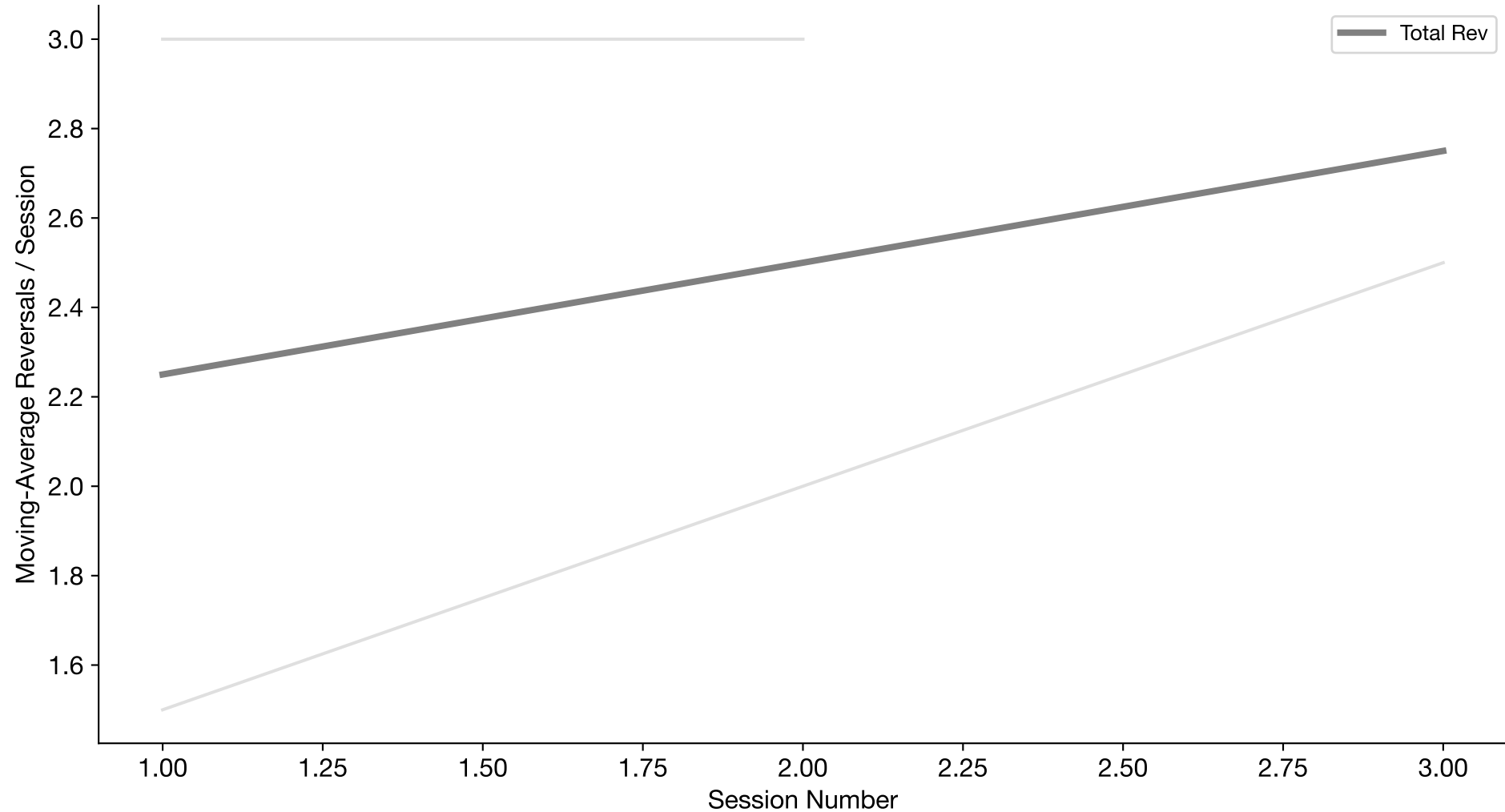
Moving-Average Total Reversals Over Time (n=2 subjects; sessions per subject=2-3; window=3)
